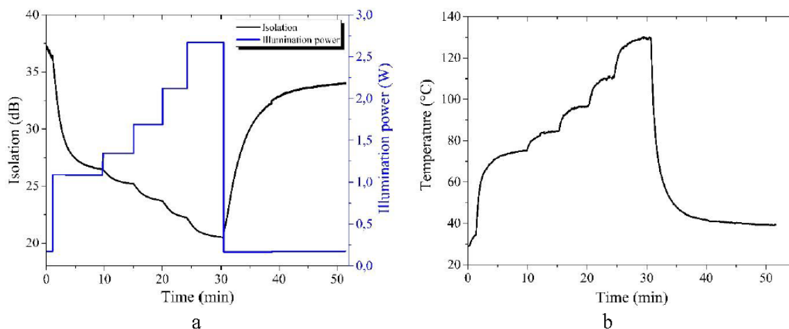
Figure 1: The typical dependencies of sample properties: (a) — isolation, (b) — temperature.
